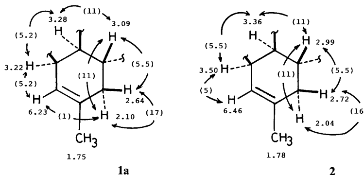
Fig. 3. 1 H-NMR Chemical Shifts (ppm) and Coupling Constants (Hz) of D-Ring Protons of Mulberrofuran F Pentamethyl Ether ( 1a ) and Mulberrofuran G ( 2 )
