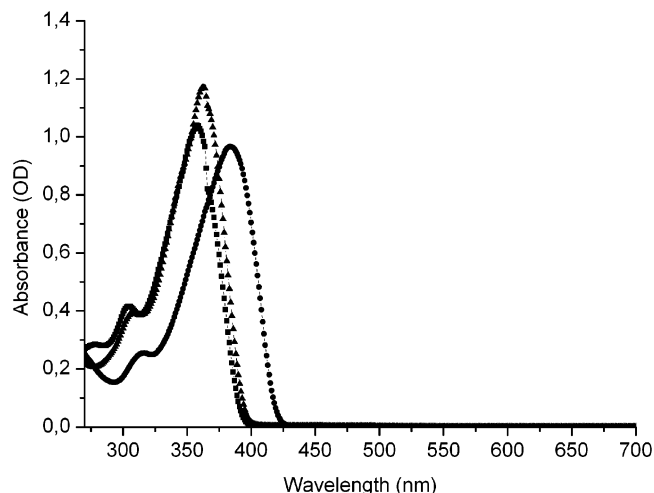
Figure 4. Absorption spectra of 10 \mu M solutions of 1 (circles), 2 (triangles), and 4 (squares) in THF.
