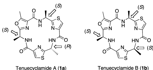
Figure 1. Structure of tenuecyclamide A (1a) and B (1b).
