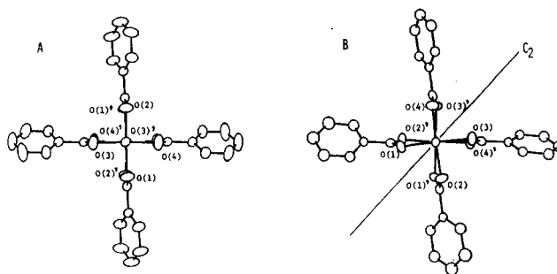
Figure 2. Views of the central regions of the \text{V}_2(\text{O}_2\text{CPh})_4\text{X}_2 molecules along the V-V' vector: (a) X = \text{C}_5\text{H}_5^- ; (b) X = \text{C}_5(\text{CH}_3)_5^- .
