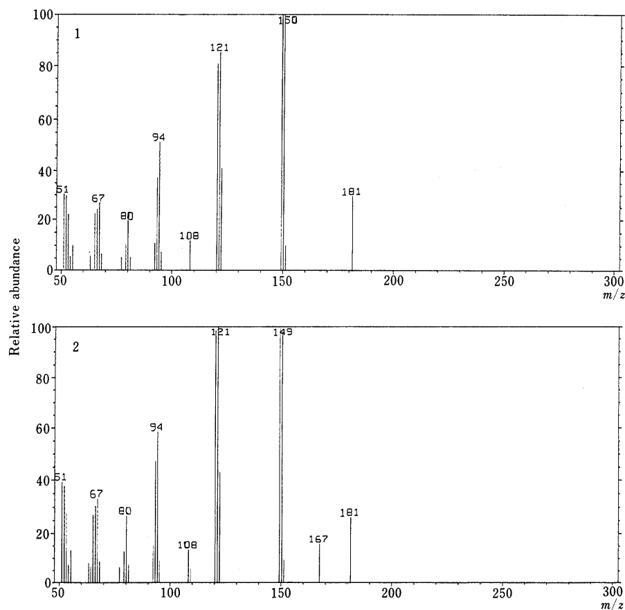
Fig. 1. Mass Spectra of (1) Pyridoxal Monomethylacetal and (2) the Solvation Product of Pyridoxal in Methanol
