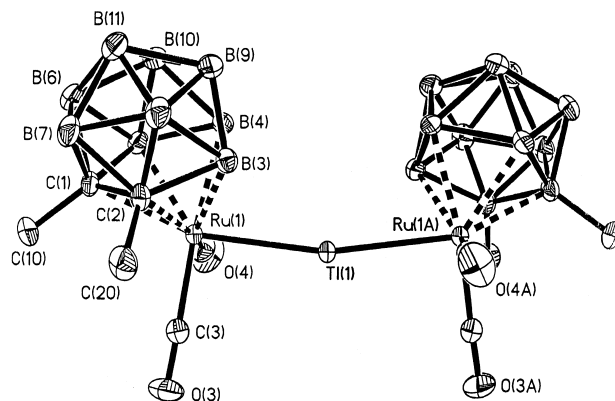
Fig. 1. Structure of the anion of [NEt 4 ][Ru 2 ( \mu -Tl)(CO) 4 ( \eta^5 -7,8-Me 2 -7,8-C 2 B 9 H 9 ) 2 ] ( 2b ), showing the crystallographic labeling scheme. Hydrogen atoms are omitted for clarity and thermal ellipsoids are shown at the 40% probability level.
