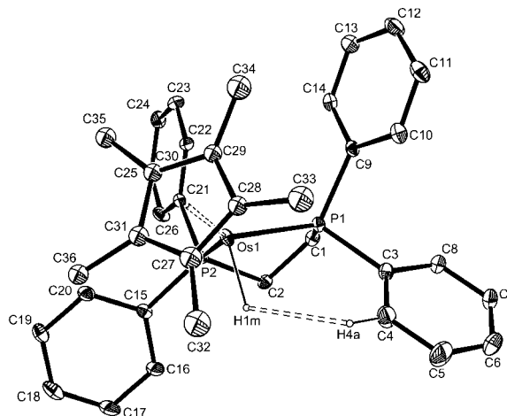
Figure 2. Molecular structure of \text{Cp}^*\text{Os}(\text{dppe})\text{H} ( 1 ) (30% probability level). Key bond lengths ( \text{\AA} ) and angles ( ^\circ ): Os–H 1.56; Os–C(NT) 1.90(3); Os–P(1) 2.2357(9); Os–P(2) 2.2302(10); CNT–Os–H 119(3); CNT–Os–P(1) 134.0(4); CNT–Os–P(2) 135(2); P(1)–M–P(2) 78.0(2).
