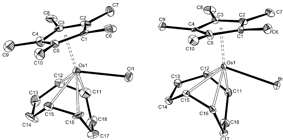
Figure 1. Molecular structures of \text{Cp}^*\text{Os}(\text{COD})\text{Cl} ( 2 ) and \text{Cp}^*\text{Os}(\text{COD})\text{Br} ( 3 ) (30% probability level). Key bond lengths (Å) and angles (deg): 2 , \text{Os}-\text{Cl} , 2.456(2); \text{Os}-\text{CNT} , 1.925(4); \text{Os}-\text{C}_{\text{av}} , 2.181(10); \text{CNT}-\text{Os}-\text{Cl} , 110.8(1); \text{Cl}-\text{Os}-\text{C}(11) , 79.9(3); \text{Cl}-\text{Os}-\text{C}(12) , 115.2(2); \text{Cl}-\text{Os}-\text{C}(15) , 119.5(2); \text{Cl}-\text{Os}-\text{C}(16) , 81.0(3); 3 , \text{Os}-\text{Br} , 2.5780(8); \text{Os}-\text{CNT} , 1.912(4); \text{Os}-\text{C}_{\text{av}} , 2.173(9); \text{CNT}-\text{Os}-\text{Br} , 110.7(1); \text{Br}-\text{Os}-\text{C}(11) , 78.0(2); \text{Br}-\text{Os}-\text{C}(12) , 112.9(3); \text{Br}-\text{Os}-\text{C}(16) , 83.8(2).
