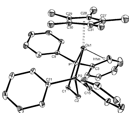
Figure 2. Molecular structure of \text{Cp}^*\text{Os}(\text{dppe})\text{H} ( 1 ) (30% probability level). Key bond lengths ( \text{\AA} ) and angles ( ^\circ ): Os–H 1.56; Os–C(NT) 1.90(3); Os–P(1) 2.2357(9); Os–P(2) 2.2302(10); CNT–Os–H 119(3); CNT–Os–P(1) 134.0(4); CNT–Os–P(2) 135(2); P(1)–M–P(2) 78.0(2).
