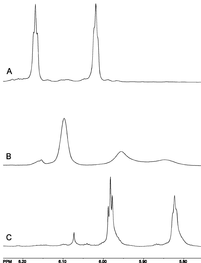
Figure 1. 1 H NMR spectra (C 5 H 4 Me region) of [Cp' 2 ZrPh] + [B(C 6 F 5 ) 4 ] − ( 2e ). Spectrum A: in CD 2 Cl 2 at −95 °C; spectrum B: in C 6 D 5 Cl/CD 2 Cl 2 at −90 °C; spectrum C: in C 6 D 5 Cl/CD 2 Cl 2 at −30 °C.
