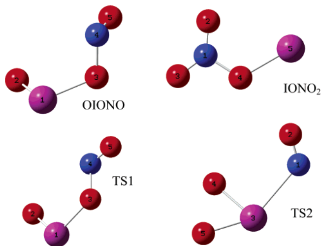
Figure 4. Geometries of stationary points on the \text{OIO} + \text{NO} potential-energy surface. The geometries are listed in Z matrix format in Table 2, and their relative energies are illustrated in Figure 5.
