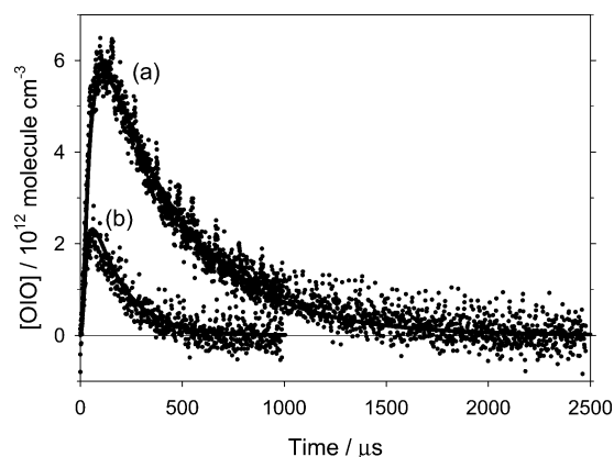
Figure 1. Typical OIO time profiles measured by CRD during the study of the reaction of OIO + NO. Experimental conditions: (a) [\text{NO}] = 2.78 \times 10^{14} \text{ molecule cm}^{-3} and (b) [\text{NO}] = 8.94 \times 10^{14} \text{ molecule cm}^{-3} ; [\text{CF}_3\text{I}] = 1.34 \times 10^{16} \text{ cm}^{-3} ; [\text{N}_2\text{O}] = 9.45 \times 10^{16} \text{ cm}^{-3} ; [\text{N}_2] = 5.34 \times 10^{17} \text{ cm}^{-3} ; T = 300 \text{ K} . The solid lines are model calculations, which include a value for k_3 of 6.0 \times 10^{-12} \text{ cm}^3 \text{ molecule}^{-1} \text{ s}^{-1} obtained by fitting a single exponential to the OIO decay an appropriate interval after the peak (see text). The concentration of OIO is derived from the model assuming a branching ratio for OIO formation from the IO self-reaction of 0.32.
