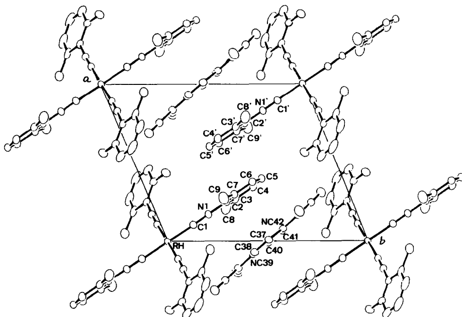
Fig. 5. The stacking arrangement in the crystals of [\text{Rh}(2,6\text{-Me}_2\text{C}_6\text{H}_3\text{NC})_4]^+\text{ATCNQ}^- as viewed normal to an ab plane. Thermal ellipsoids are drawn at the 20% probability.
