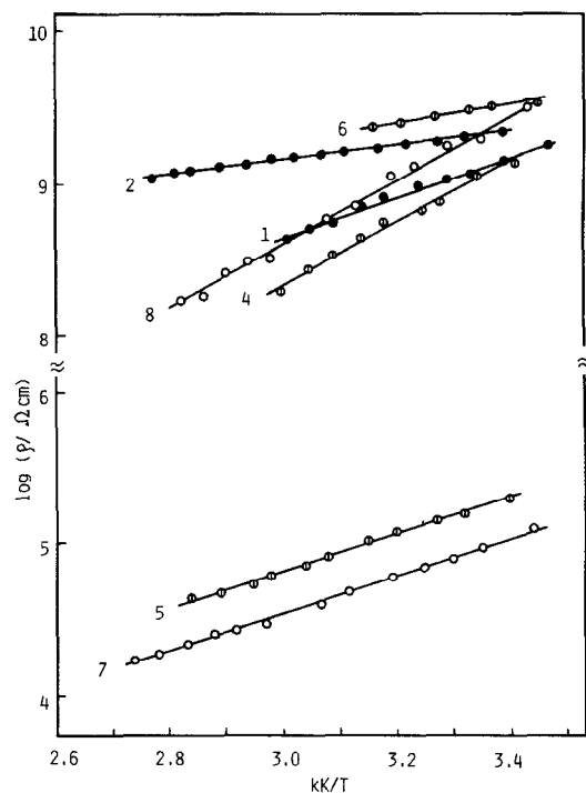
Fig. 4. Temperature dependence of the specific resistivity of the \text{Rh(I)}-\text{ATCNQ}^- and \text{Rh(I)}-\text{ATCNQ}^-/\text{TCNQ}^-/\text{TCNQ} salts.
