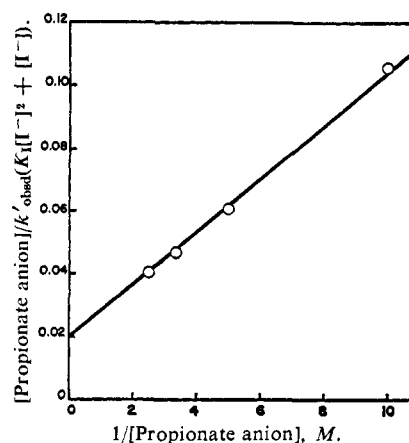
Figure 5. Plot of the left-hand side of relationship 16 against 1/[\text{propionate anion}] for the oxidation of tetrahydrothiophene ( 1.3 \times 10^{-3} M ) by iodine (initial [I_2]_T = 1 \times 10^{-4} M ; [KI] = 1 \times 10^{-2} M ) in various propionate buffers at pH 4.80 and 25^\circ .
