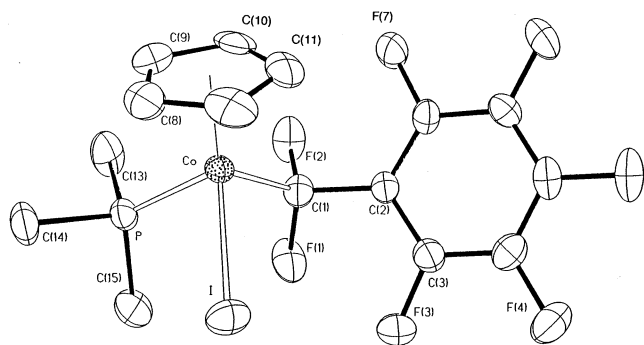
Figure 1. ORTEP drawing and labeling scheme for 3a . Ellipsoids are drawn at 35% probability. Hydrogens have been omitted for clarity.
