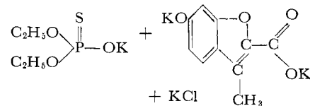
Reaction II
