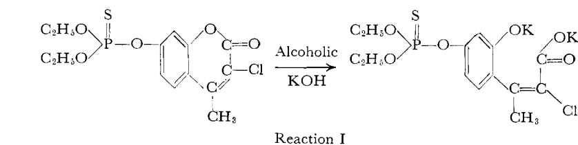
Reaction I
