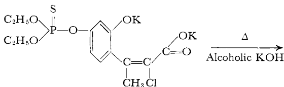
Reaction I
