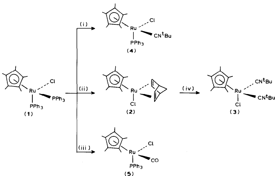
SCHEME 1. (i) \text{Bu}^t\text{NC} , \text{CH}_2\text{Cl}_2 , 20^\circ\text{C} ; (ii) norbornadiene, \text{C}_7\text{H}_8 , 100^\circ\text{C} ; (iii) \text{HCO}_2\text{H} , \text{C}_7\text{H}_8 , 140^\circ\text{C} ; (iv) \text{Bu}^t\text{NC} , \text{C}_7\text{H}_8 , 100^\circ\text{C} .
