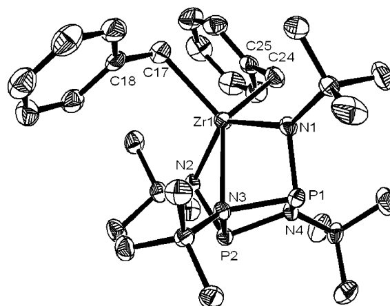
Figure 2. ORTEP plot of [( t -BuN)( t -BuNP) 2 ] 2 Zr(CH 2 Ph) 2 ( 14 ) with thermal ellipsoids drawn at the 50% probability level. All hydrogen atoms were omitted for clarity.
