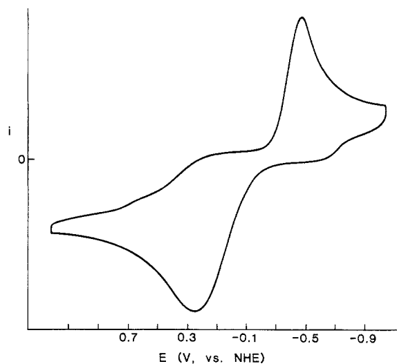
Figure 2. A cyclic voltammogram of [Os(NH _3 ) _5 (CH _3 ) _2 CO] ^{2+} in 0.5 N TBAH. Scan rate = 100 mV/s.
