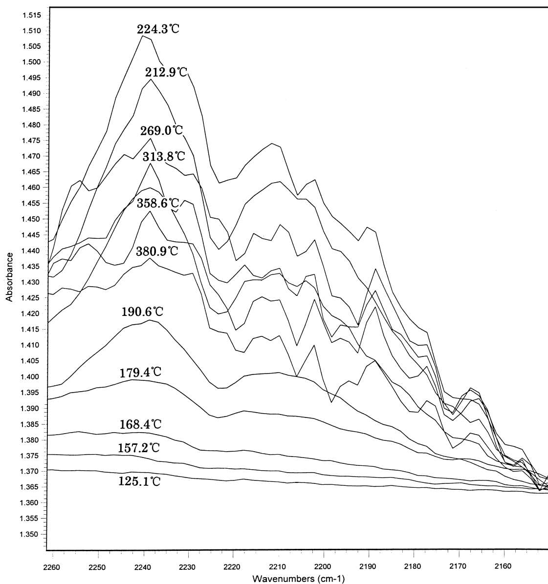
Fig. 4. Characteristic absorption peak of product \text{N}_2\text{O} at various temperatures.
