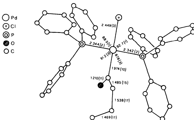
Fig. 1. Molecular structure of trans - \text{Pd}(\text{COPr-n})\text{Cl}(\text{PPh}_3)_2 . Hydrogen atoms are omitted.
