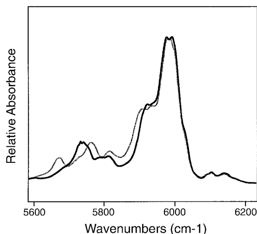
Figure 1. Room-temperature vapor phase overtone spectrum of toluene- \alpha - d_1 (solid line) in the \Delta\nu_{CH} = 2 region measured with a path length of 11.25 m and a pressure of 17 Torr. The scaled spectrum of toluene- d_0 (dotted line) is taken from ref 1 (see text).
