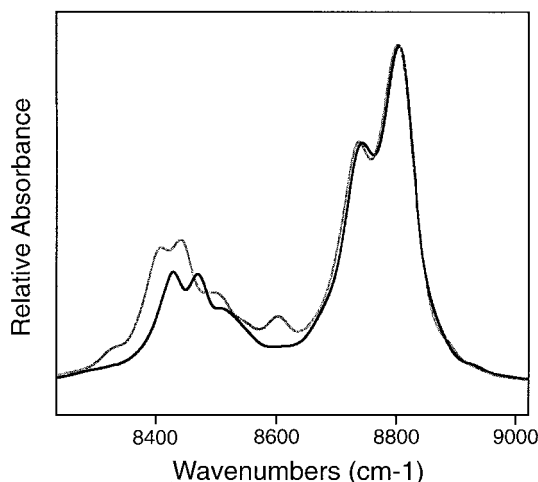
Figure 2. Room-temperature vapor phase overtone spectrum of toluene- \alpha - d_1 (solid line) in the \Delta\nu_{CH} = 3 region measured with a path length of 11.25 m and a pressure of 17 Torr. The scaled spectrum of toluene- d_0 (dotted line) is taken from ref 1 (see text).
