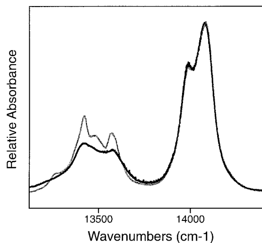
Figure 4. Room-temperature vapor phase overtone spectrum of the toluene- \alpha - d_1 (solid line) in the \Delta\nu_{CH} = 5 region. The spectrum was measured by ICL-PAS with a sample pressure of 16 Torr. The scaled spectrum of toluene- d_0 (dotted line) is taken from ref 1 (see text).
