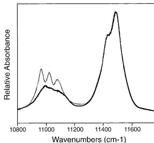
Figure 3. Room-temperature vapor phase overtone spectrum of toluene- \alpha - d_1 (solid line) in the \Delta\nu_{CH} = 4 region. The spectrum was measured by ICL-PAS with a sample pressure of 17 Torr of toluene- \alpha - d_1 and 100 Torr of argon buffer gas. The scaled spectrum of toluene- d_0 (dotted line) is taken from ref 1 (see text).
