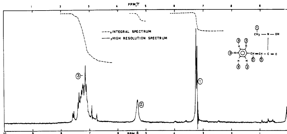
Figure 1. ^1\text{H} NMR spectrum of N -methylcinnamohydroxamic acid in \text{CDCl}_3 .
