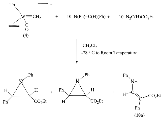
Scheme 4. Catalytic Aziridine Formation
