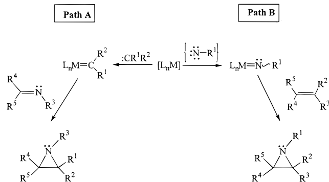
Scheme 3. Two Methodologies for Aziridine Synthesis a
