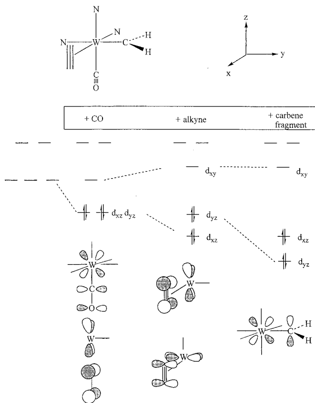
Scheme 2. Qualitative Molecular Orbital Diagram for [\text{Tp}^*(\text{CO})(\text{PhC}\equiv\text{CR})\text{W}=\text{CH}_2][\text{PF}_6] ( 3 ) and ( 4 ) ( \text{R} = \text{Ph}, \text{Me}; \text{Tp}^* = \text{Tp}, \text{Tp}' )
