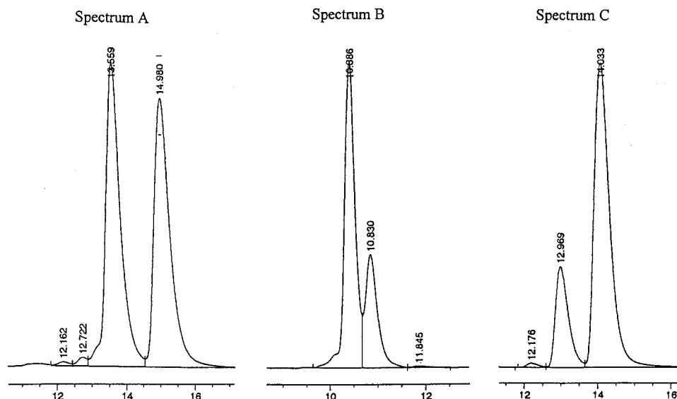
Figure 3. Determination of % ee for enriched \text{Tp}'(\text{CO})(\text{PhC}\equiv\text{CMe})\text{W}-\text{Me} ( 1 ) Using Chiral HPLC: spectrum A, racemic mixture; spectrum B, produced from RS -amine; spectrum C, produced from SS -amine (configuration at metal center given first, see ref 32).
