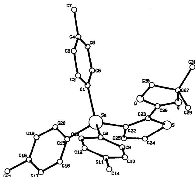
Fig. 1. [2-(4,4-Dimethyl-2-oxazoliny-3-thienyl)tri( p -tolyl)]tin. Selected bond distances ( \text{\AA} ) and angles ( ^\circ ): Sn-O 2.977(3), Sn-C(1) 2.134(4), Sn-C(8) 2.124(4), Sn-C(15) 2.144(4), Sn-C(22) 2.151(4); C(1)-Sn-C(8) 112.5(2), C(1)-Sn-C(15) 107.2(2), C(1)-Sn-C(22) 108.5(2), C(8)-Sn-C(15) 109.5(2), C(8)-Sn-C(22) 113.5(2), C(15)-Sn-C(22) 105.2(2).
