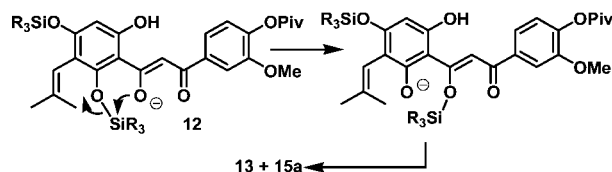
Scheme 4. Possible Mechanism for the Desilylation of the Diaryl methane 12 by Lewis Acids (R = tert -Butyldimethylsilyl)
