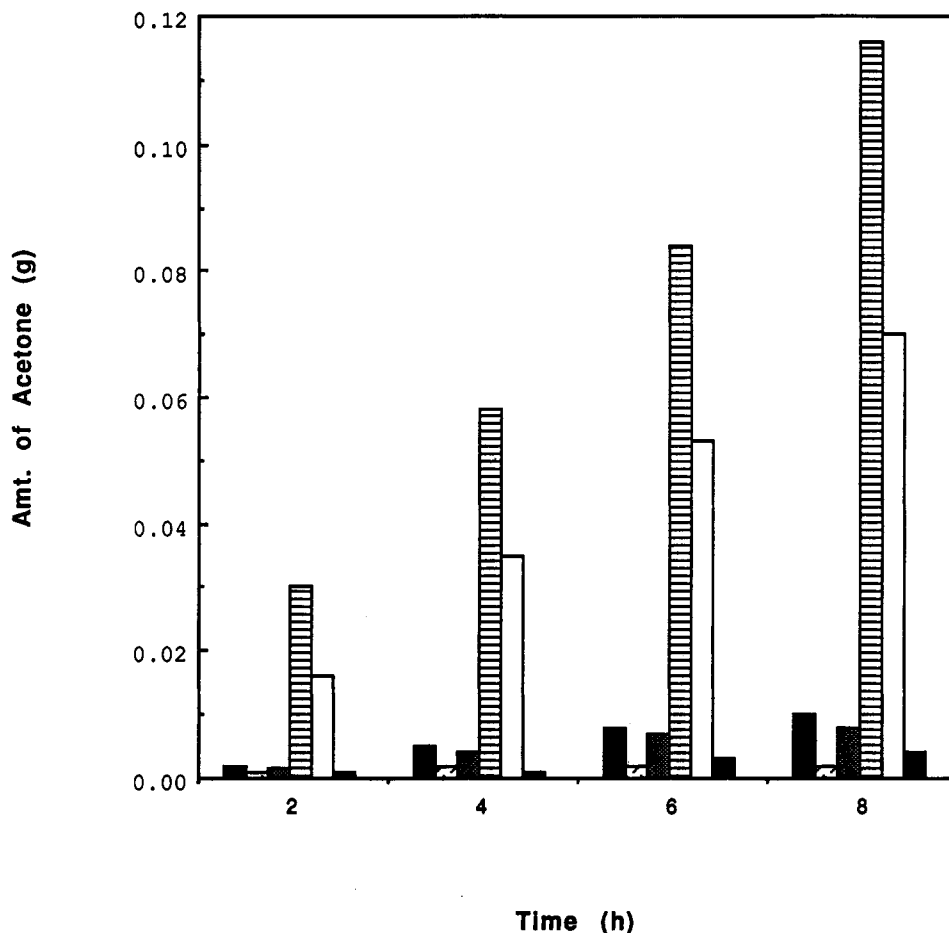
Figure 3. Yields for manganese oxide catalysts at 2, 4, 6, and 8 h from left to right: hollandite; cryptomelane; todorokite; A-MnO 2 ; commercial A-MnO 2 (<80 \mu m); commercial A-MnO 2 (>80 \mu m).
