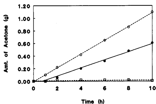
Figure 6. Effect of prephotolysis and oxygen on manganese oxide catalysts: (O) fresh catalyst photolyzed in oxygen; (●) prephotolyzed 1 h in O 2 ; (□) prephotolyzed 1 h in N 2 .
