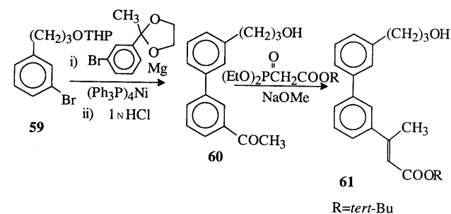
Chart 6. Synthesis of Propanol 61
