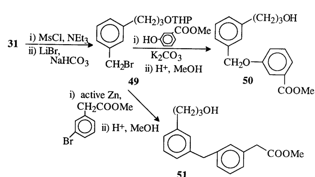
Chart 4. Synthesis of Propanols 50 and 51
