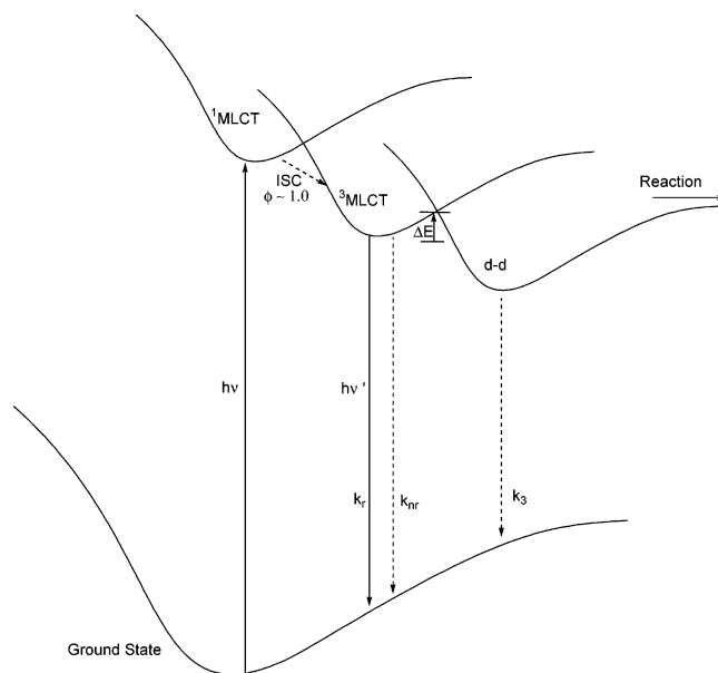
Figure 8. Schematic diagram of the photophysical processes of Ru(bpy) 3 2+ . 40
