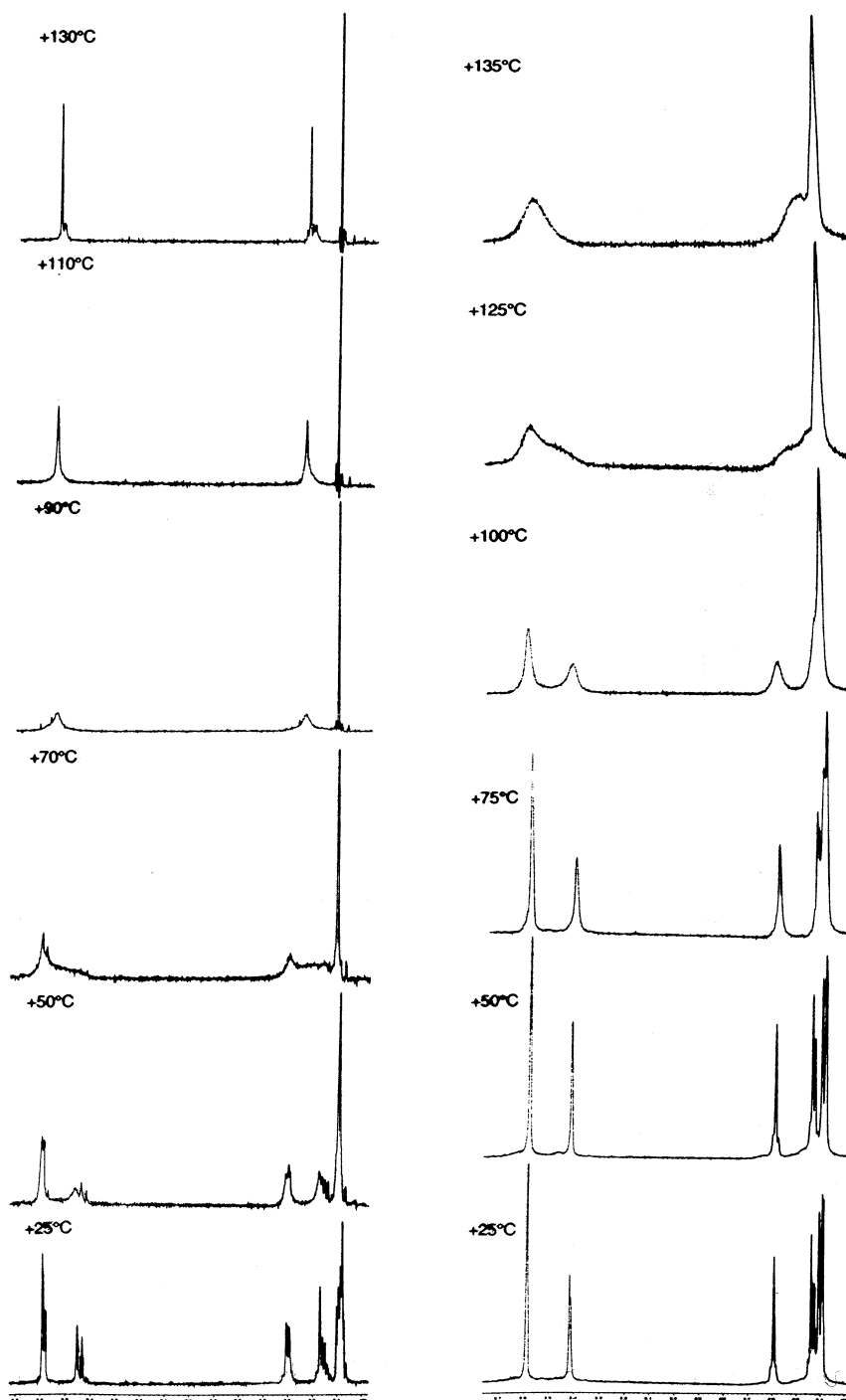
Fig. 4. 1 H-NMR variable temperature experiments of (Q D ) 2 SnF 2 (a) and of (Q D ) 2 SnCl 2 (b).
