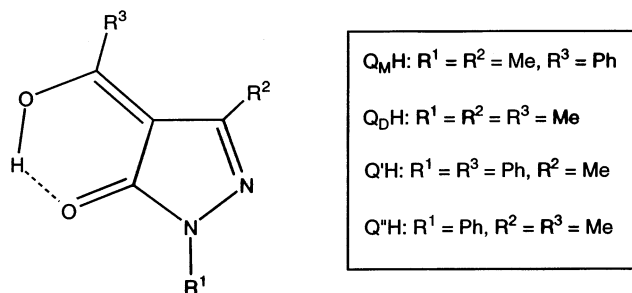
Fig. 1. 4-Acyl-5-pyrazolone proligands.
