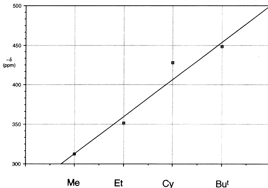
Fig. 6. The effect of increasing substitution of R on the ^{119}\text{Sn} chemical shift of (\text{Q}_\text{D})_2\text{SnR}_2 ( \text{R} = \text{Me}, \text{Et}, \text{Cy}, \text{Bu}' ).
