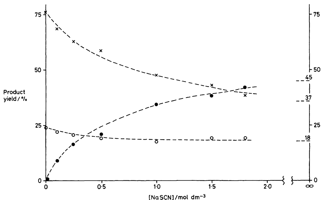
Figure 1. Product yields from solvolysis of ( 1a ) in 1:1 (v/v) \text{H}_2\text{O} : \text{CF}_3\text{CH}_2\text{OH} containing NaSCN \times = \text{PhCH}_2\text{OH} ; \circ = \text{PhCH}_2\text{OCH}_2\text{CF}_3 ; \bullet = \text{PhCH}_2\text{SCN} .
