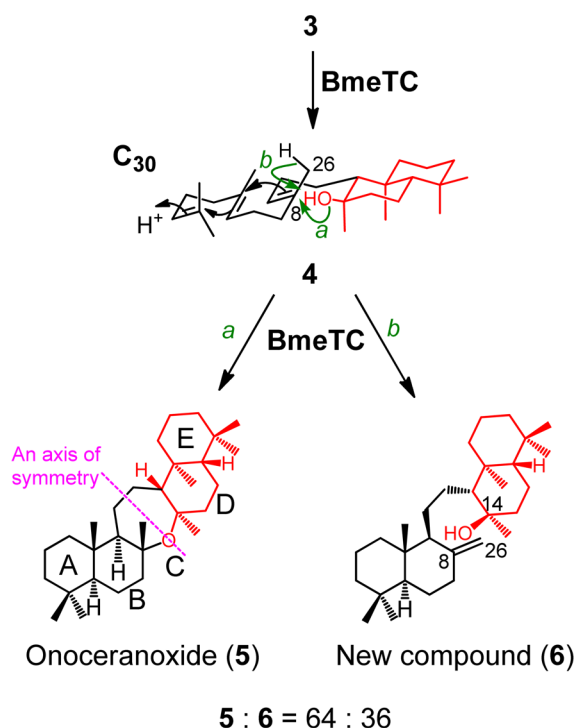
Scheme 2. Cyclization of Bicyclic Triterpene (4) into Onocerooids 5 and 6 Catalyzed by BmeTC a
