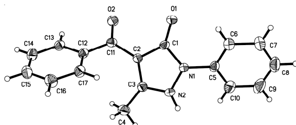
Fig. 1. Molecule structure of the title compound
