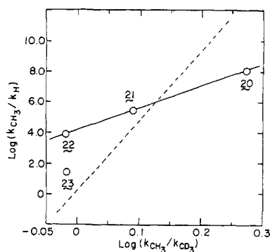
Figure 1. Plot of \log(k_{\text{CH}_3}/k_{\text{H}}) vs. \log(k_{\text{CH}_3}/k_{\text{CD}_3}) for 7-norbornyl tosylates (20), syn-7-norbornenyl tosylates (21), and anti-7-norbornenyl tosylates (22) represented by solid line. For purposes of comparing our slope with that of Sunko and coworkers (ref 35), their line for the solvolysis of a variety of chlorides is included (-----).
