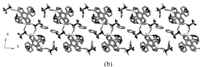
Figure 5. (a) View of twin chain formed by linking a single chain through the \text{Ag}-(\text{SO}_3\text{CF}_3)_2-\text{Ag} linkage. (b) Twin chains arranged one by one along the b axis, with benzene molecules filling in the clearance.
