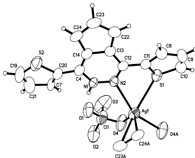
Figure 8. Coordination environment of \text{Ag(I)} in 4 .
