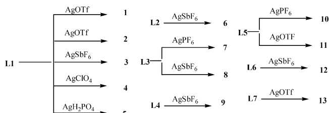
Scheme 2. Synthesis of Ag(I)–Fulvene Complexes
