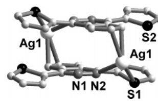
Figure 9. Boxlike moiety in compound 4 .
