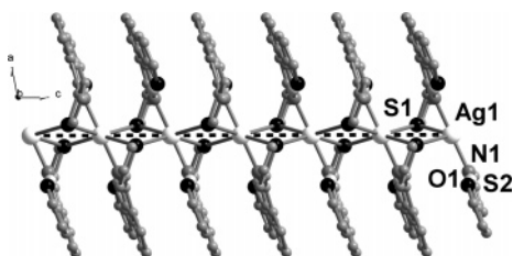
Figure 14. One-dimensional chain in 6 driven by Ag \cdots S and \pi - \pi interactions.
