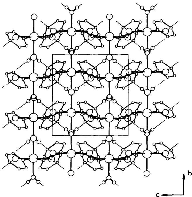
Fig. 2. Projection of the unit cell contents for \text{Ph}_2\text{SbCl}_3 \cdot \text{H}_2\text{O} down the a axis; hydrogen bonds are shown as weak lines.
