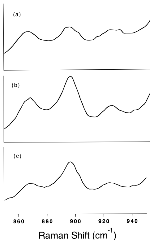
Figure 7. Resonance Raman spectra of \text{Sm}(\text{SePh})_3 (adsorption \lambda_{\text{max}} = 425 \text{ nm} ) dissolved in pyridine, between 850 and 950 \text{cm}^{-1} taken at room temperature. The laser energy decreases from top to bottom. Note the clear enhancement of the mode at 900 \text{cm}^{-1} . Key: (a) 488.0 nm (2.54 eV); (b) 514.5 nm (2.41 eV); (c) 568.2 nm (2.18 eV).
