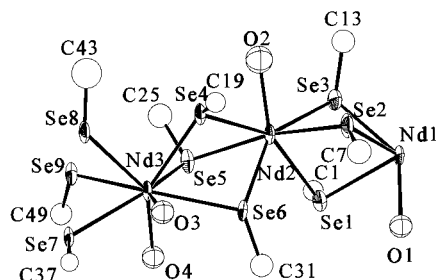
Figure 6. Molecular structure of the repeating unit in polymeric [(THF)_4Nd_3(SePh)_9]_n with most of the C and H atoms removed for clarity.
