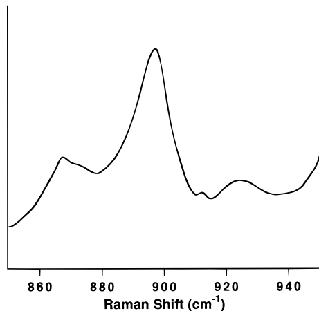
Figure 8. Resonance Raman spectra of \text{Yb}(\text{SePh})_3 (adsorption \lambda_{\text{max}} = 510 \text{ nm} ) dissolved in pyridine, between 850 and 950 \text{cm}^{-1} using a 514.5 nm (2.34 eV) laser excitation at room temperature. Note the clear enhancement of the mode at 900 \text{cm}^{-1} .
