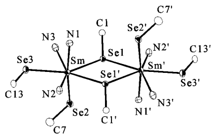
Figure 5. Molecular structure of dimeric [(py)_3Sm(SePh)_3]_2 with most of the C and H atoms removed for clarity.
