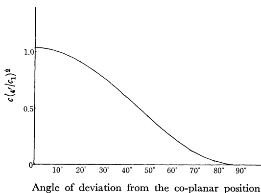
Fig. 2. Relation between (c_{4'}/c_1)^2 and angle of deviation from the co-planar position.
