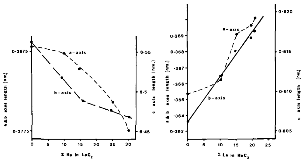
FIG. 3. Unit cell a , b , and c parameters as a function of composition in \text{Ho}_{1-x}\text{La}_x\text{C}_2 through the two tetragonal phase regions.
