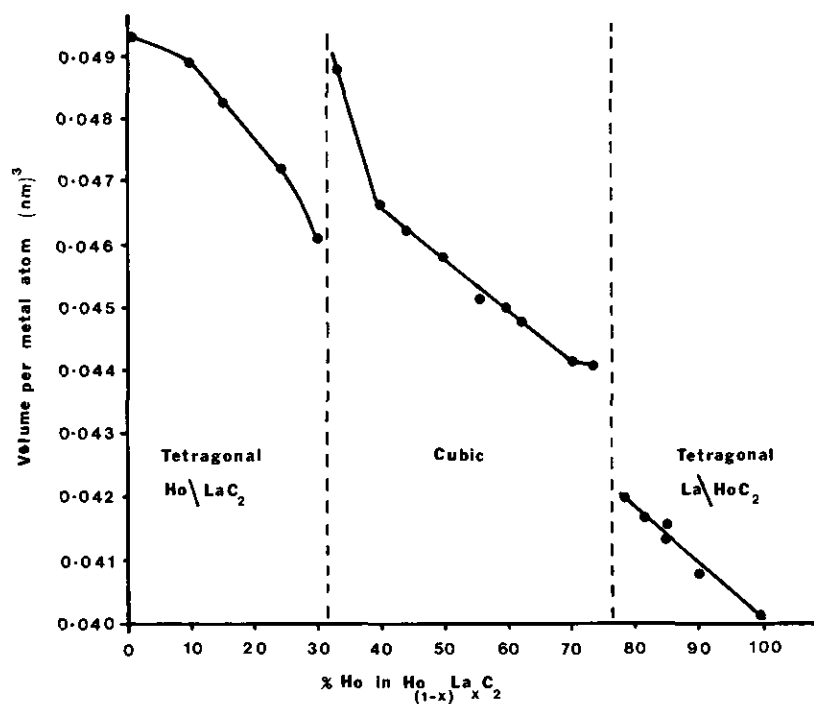
FIG. 2. Volume per metal atom in the unit cell of \text{Ho}_{1-x}\text{La}_x\text{C}_2 solid solutions.
