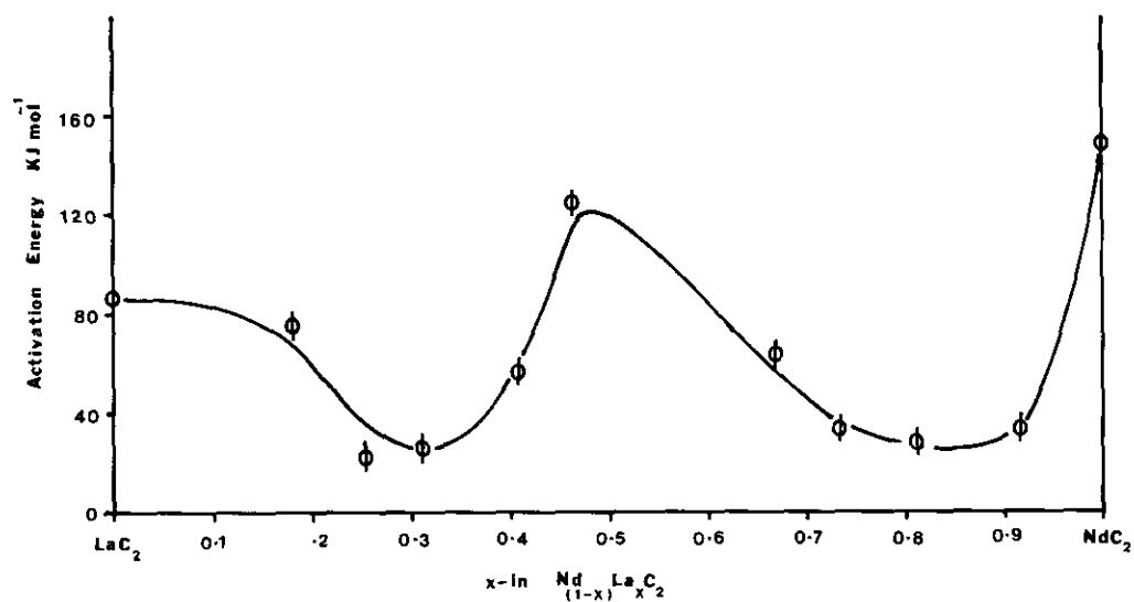
FIG. 9. Hydrolysis reaction activation energies for a series of \text{Nd}_{1-x}\text{La}_x\text{C}_2 solid solutions.
