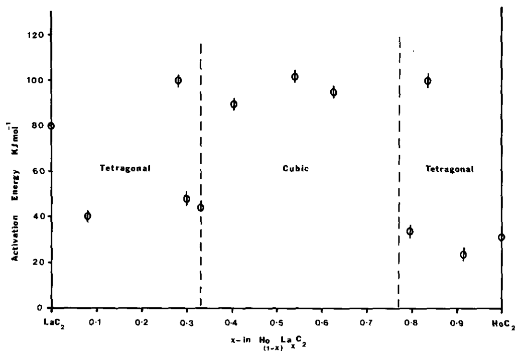
FIG. 8. Hydrolysis reaction activation energies for a series of \text{Ho}_{1-x}\text{La}_x\text{C}_2 solid solutions.
