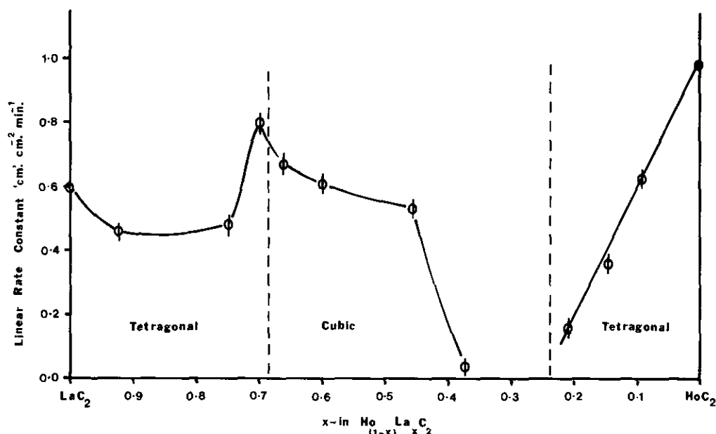
FIG. 6. Variation in linear rate constant with composition at 20°C for the \text{Ho}_{1-x}\text{La}_x\text{C}_2 series of solid solutions.
