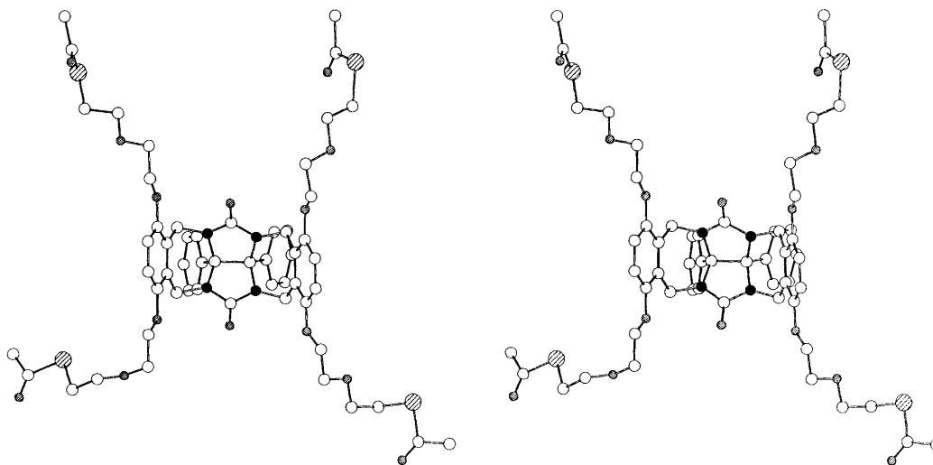
Fig. 1 Stereoview of 1a
