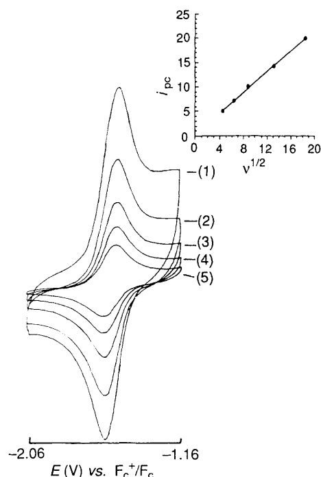
Fig. 2 Cyclic voltammograms of cluster compound 2 recorded as a function of the scan rate v ; 400 \text{mV s}^{-1} (1), 200 \text{mV s}^{-1} (2), 100 \text{mV s}^{-1} (3), 50 \text{mV s}^{-1} (4), 25 \text{mV s}^{-1} (5). Measurements were conducted at ca. 25°C in DMF using a platinum disk working electrode, a platinum auxiliary electrode and Ag/AgCl reference electrode (0.32 \text{mmol dm}^{-3} of cluster compound 2 , 0.1 \text{mol dm}^{-3} tetrabutylammonium hexafluorophosphate (TBAH) as the supporting electrolyte, 20 \text{mmol dm}^{-3} \text{Ba}(\text{ClO}_4)_2 as modulator). Inset: plot of the peak current for the reduction process at the Pt-electrode vs. the square-root of the scan rate, v^{1/2} , verifying the predominance of linear diffusion for cluster compound 2 .
