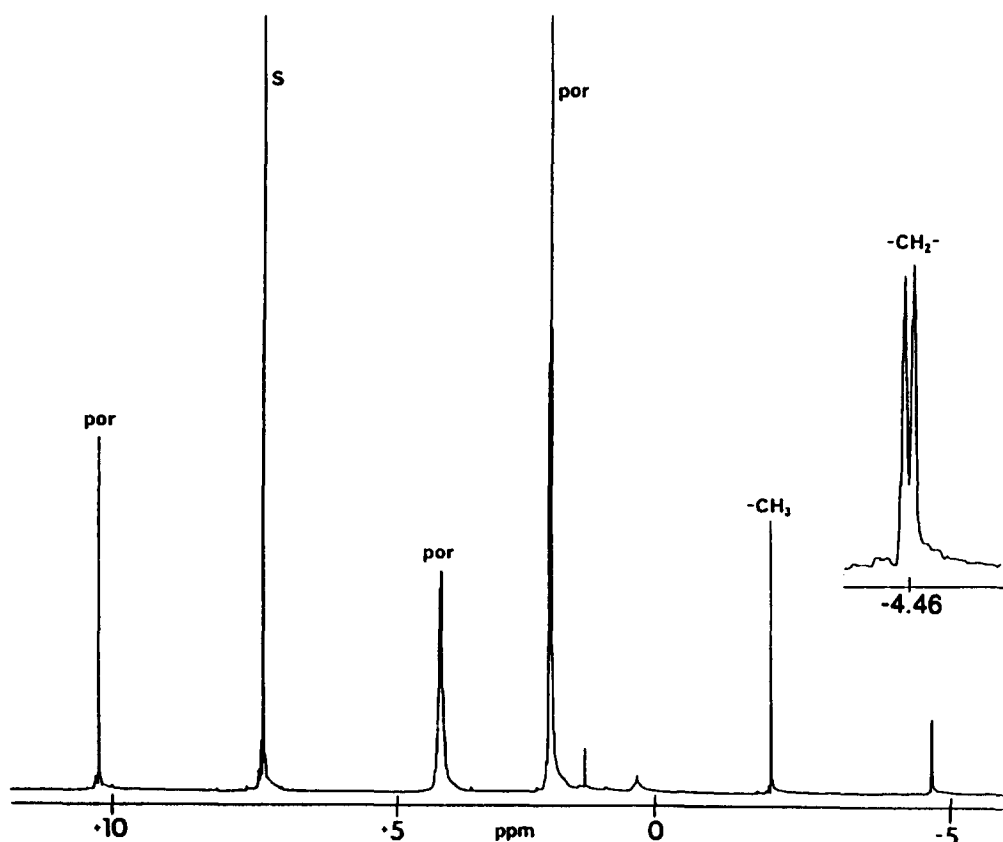
Fig. 2. Proton NMR spectrum for compound 16 , (OEP)Rh–CH 2 C(O)CH 3 , in C 6 D 6 . Inset: expanded high field region.
