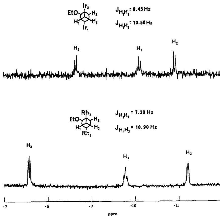
Fig. 5. High field proton NMR spectra for ethoxy substituted \{\mu\text{-CH}_2\text{CH}(\text{X})\}[(\text{OEP})\text{M}]_2 complexes ( 19a , \text{M} = \text{Rh} ; 19b , \text{M} = \text{Ir} ) in \text{C}_6\text{D}_6 .
