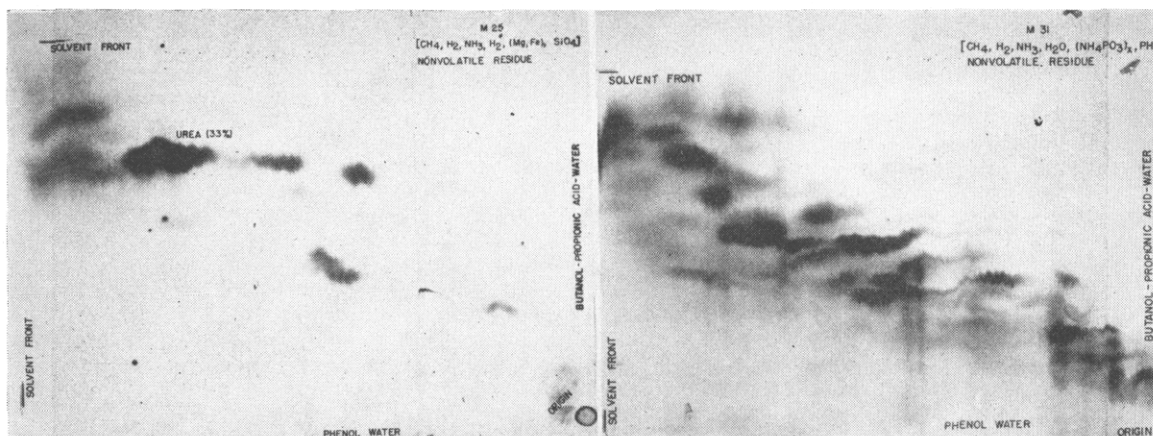
Fig. 2. a —Chromatograms of experiments M25 and M31.
