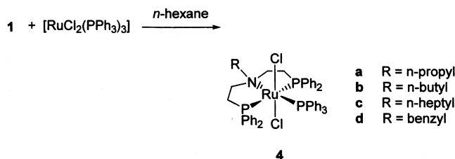
Scheme 2. Coordination of PNP Ligands to [RuCl 2 (PPh 3 ) 3 ]
