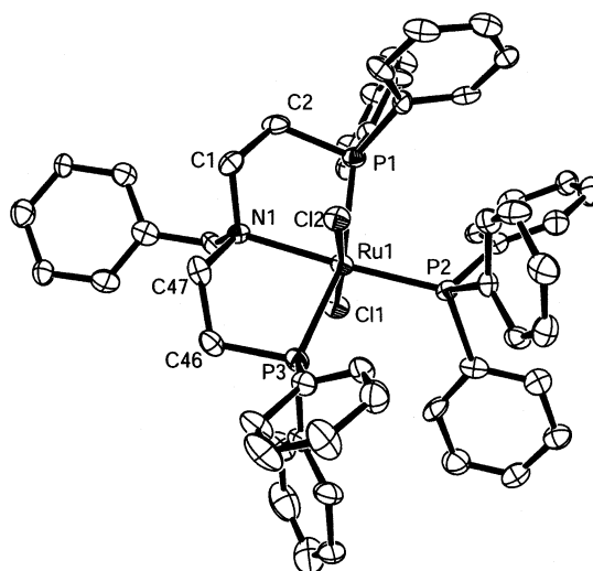
Figure 1. ORTEP diagrams of complexes 4b (left) and 4d (right) at 50% probability. Solvent molecules and hydrogen atoms are omitted for clarity.
