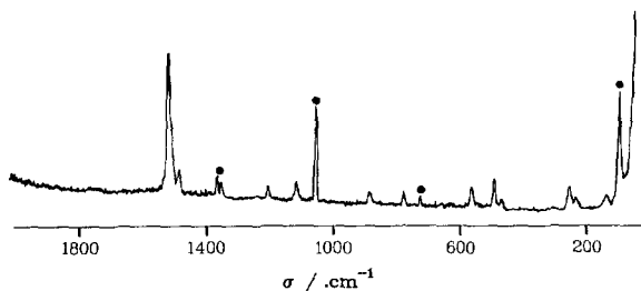
Fig. 8 Resonance Raman spectrum of [\text{Ph}_3\text{SnRe}(\text{CO})_3(\text{t-Bu-DAB})] ( \text{KNO}_3 disk at 110 K; \lambda_{\text{exc}} = 514.5 nm; p = 120 mW).
