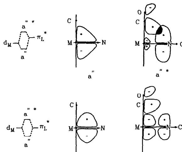
Fig. 9. Excited state 'through-space' interaction of metal d_\pi , \alpha -diimine \pi^*_1 and axial carbonyl \pi^* orbitals in the case of the weak (top) and strong (bottom) metal ( d_\pi )– \alpha diimine ( \pi^*_1 ) mixing.
