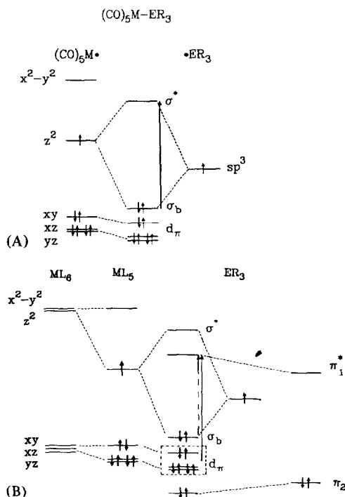
Fig. 3. (A): qualitative molecular orbital diagram of [\text{R}_3\text{EM}(\text{CO})_5] ; (B): qualitative molecular orbital diagram of [\text{R}_3\text{EM}(\text{CO})_3(\alpha\text{-diimine})] .
