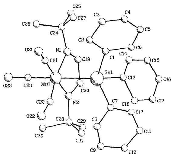
Fig. 4. PLUTO drawing of [\text{Ph}_3\text{SnMn}(\text{CO})_3(\text{t-Bu-DAB})] .
