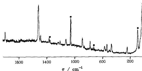
Fig. 7. Resonance Raman spectrum of [\text{Ph}_3\text{SnMn}(\text{CO})_3(\text{t-Bu-DAB})] ( \text{KNO}_3 disk at 110 K; \lambda_{\text{exc}} = 514.5 nm; p = 100 mW).
