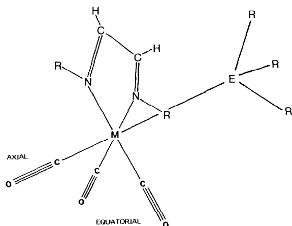
Fig. 2. General molecular geometry of the complexes [Ph_3EM(CO)_3(\alpha\text{-diimine})] .
