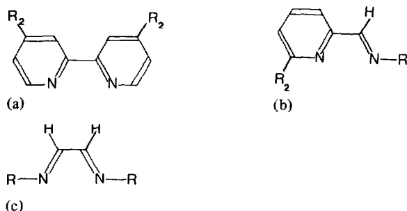
Fig. 1. \alpha -diimines: 2,2'-bipyridine (a) (bipy, R_2 = H ; bipy', R_2 = CH_3 ), pyridine-2-carbaldehydeimine (b) ( R -PyCa, R_2 = H ; R -PyCa', R_2 = CH_3 ) and 1,4-diaza-1,3-butadiene (c) ( R -DAB).
