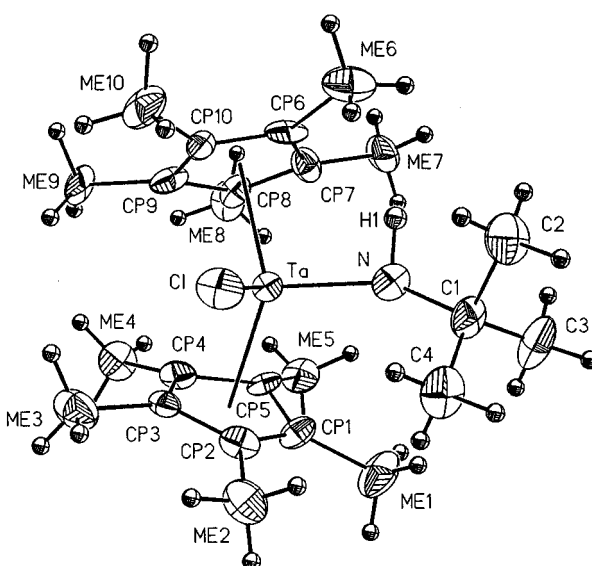
Figure 2. Drawing of the cation of [Cp* 2 Ta(NHNCMe 3 )Cl]-[B(C 6 F 5 ) 4 ] ( 3 ) (50% ellipsoids). Ta-Cp*(1) = 2.158 Å, Ta-Cp*(2) = 2.173 Å, Ta-N = 1.940(11) Å, Ta-Cl = 2.372(3) Å, N-C(1) = 1.511(14) Å, N-H(1) = 1.180(11) Å, Ta-H(1) = 2.31 Å; Cp*1-Ta-Cp*2 = 132.5°, N-Ta-Cl = 94.1(3)°, Ta-N-C1 = 155.4(9)°.
