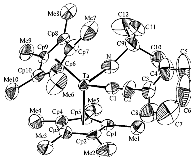
Figure 4. Drawing of the cation of [\text{Cp}^*_2\text{Ta}(\text{NHCC}_6\text{H}_5)(\text{C}\equiv\text{CC}_6\text{H}_5)][\text{B}(\text{C}_6\text{F}_5)_4] ( 7 ) (50% ellipsoids). Ta–Cp(A) = 2.157 Å, Ta–Cp(B) = 2.172 Å, Ta–N = 1.928(7) Å, Ta–C1 = 2.097(9) Å, N–C9 = 1.570(12) Å, C1–C2 = 1.202(13) Å, C2–C3 = 1.459(14) Å; Cp(A)–Ta–Cp(B) = 134.7°, N–Ta–C1 = 92.5(3)°, Ta–N–C9 = 151.8(6)°.
