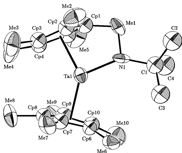
Figure 1. Drawing of the cation of [Cp*Ta( \eta^5 -C 5 Me 4 CH 2 -NCMe 3 )H][B(C 6 F 5 ) 4 ] ( 2 ) (50% ellipsoids). Ta1-Cp*(1) = 2.081 Å, Ta1-Cp*(2) = 2.131 Å, Ta1-N1 = 1.976(10) Å, N1-C1 = 1.555(17) Å, N1-Me1 = 1.441(16) Å, Cp1-Me1 = 1.479(19) Å; Cp*1-Ta1-Cp*2 = 137.8°, Ta1-N1-C1 = 146.1(8)°, Ta1-N1-C1 = 108.4(9)°.
