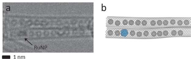
Fig. 3 (a) TEM image of two nanotubes of the RuNPs@SWNT catalyst after exposure to C 60 . (b) Structural diagram showing the positions of the C 60 molecules (grey) and the RuNP (blue) inside the carbon nanotubes.
