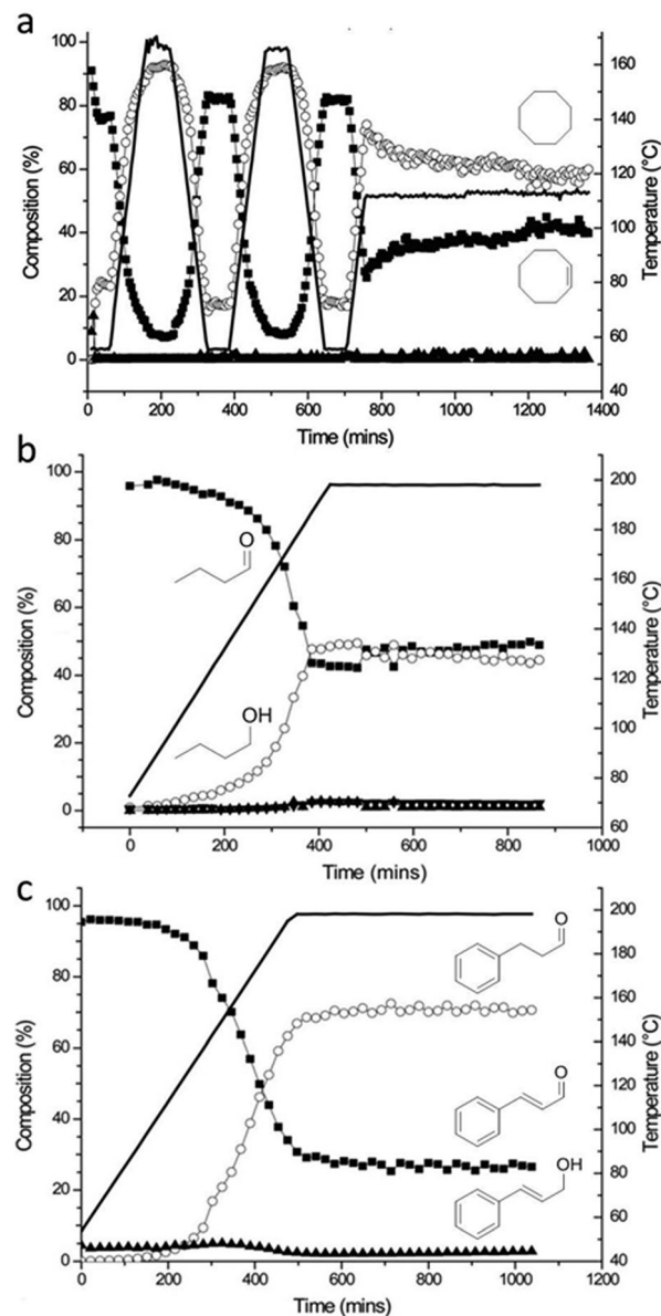
Fig. 2 Reaction kinetics for the reduction of (a) cyclooctene (■) to cyclooctane (○) and other products (▲), (b) butyraldehyde (■) to butanol (○) and small amounts of other products (▲) and then changing the feedstock solution for the reduction of (c) cinnamaldehyde (■) to hydrocinnamaldehyde (○) and cinnamyl alcohol (▲). The reactor internal temperature is shown as the solid line in all plots. Flow rates were as follows; 1 mL min -1 CO 2 , 0.03 mL min -1 organic substrate, 0.06 mL min -1 H 2 under 100 bar pressure.
