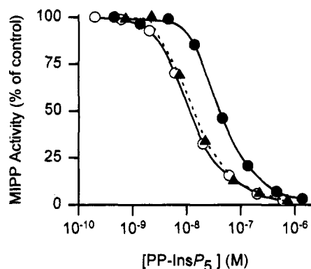
Figure 1. Inhibition of MIPP activity by PP-InsP 5 . A multiple inositol polyphosphate phosphatase (MIPP) was purified and incubated with [ 3 H]Ins(1,3,4,5)P 4 as previously described, 16 in the presence of the indicated concentrations of either 10 (○—○), 11 (●—●), or commercial PP-InsP 5 (▲—▲). The extent of MIPP-mediated hydrolysis of [ 3 H]Ins-(1,3,4,5)P 4 is plotted as a percentage of the control activity in the absence of any PP-InsP 5 .
