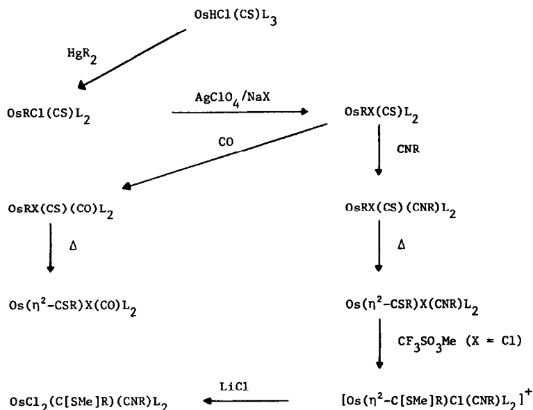
SCHEME 1. Synthesis of osmium(II) thioacyl complexes ( L = \text{PPh}_3 , R = p\text{-tolyl} , X = \text{Cl, Br, I, O}_2\text{CCF}_3 ).
