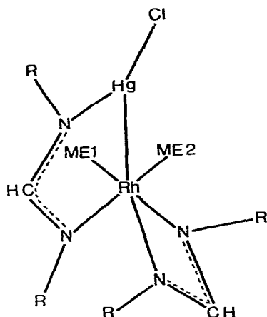
Fig. 3. Structure of [(\text{Diene})\{\text{RNC(H)NR}\}_2\text{RhHgCl}]_2 in solution ( \text{R} = (\text{CH}_3)_2\text{CH} ). \text{ME}_1 and \text{ME}_2 are the midpoints of the olefinic bonds in the COD and NOR ligands.
