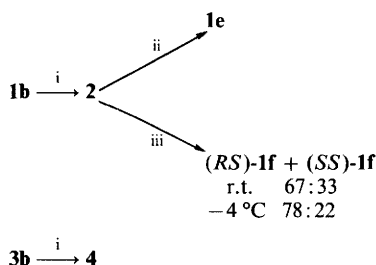
Scheme 3 Reagents [yields]: i, \text{BBr}_3 , then water; 2 [quant.], 4 [58%]; ii, \text{NaOEt} , \text{EtOH} [73%]; iii, (S)\text{-LiNHCH(Me)Ph}
