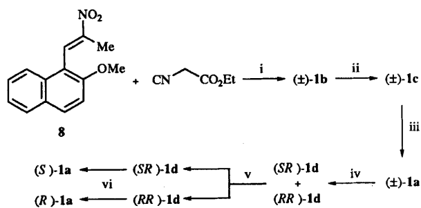
Scheme 1 Reagents and conditions [yields]: i, DBU [83%]; ii, Na-PhCH 2 OH [89%]; iii, H 2 , Pd/C [96%]; iv, (R)-PhCH(Me)OH, 2-Br-1-ethylpyridinium BF 4 - [91%]; v, crystallization; (SR)-1d [26% based on (±)-1a], then column chromatography; (RR)-1d [28% based on (±)-1a]; vi, H 2 , Pd/C
