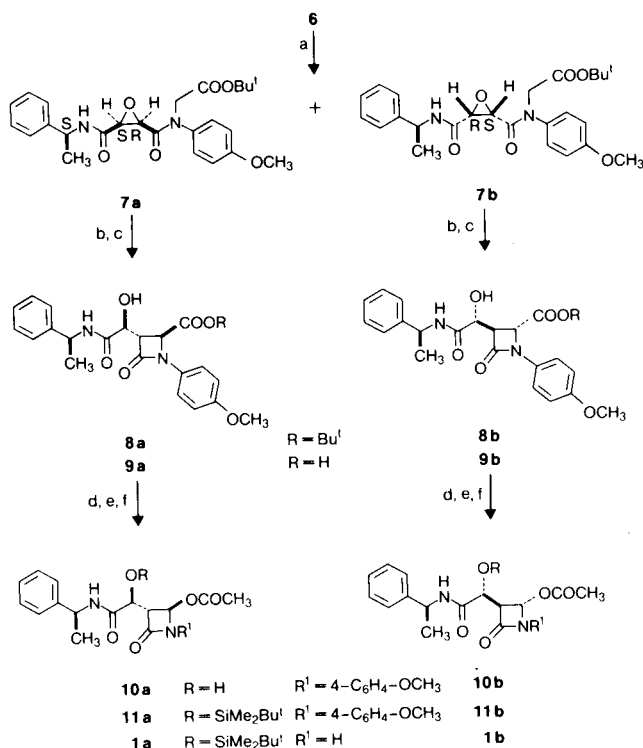
Scheme II. Elaboration of the Optically Active Acetoxiazetidinones 1a and 1b [a]
