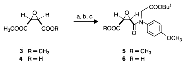
Scheme I. Preparation of the Racemic Acid 6 [a].
