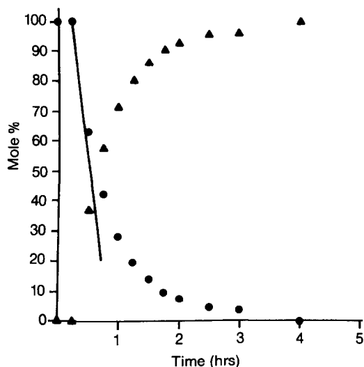
Fig. 1. Reaction profile for the hydrogenation of cis,cis -9,12-methyl linoleate (0.045 M ) under 100 p.s.i. H_2 pressure at 135°C in hexane: [Cr(naphthalene)(CO)_3]/[substrate] = 0.1 : (●) methyl linoleate and (▲) reduction products methyl iso-oleates
