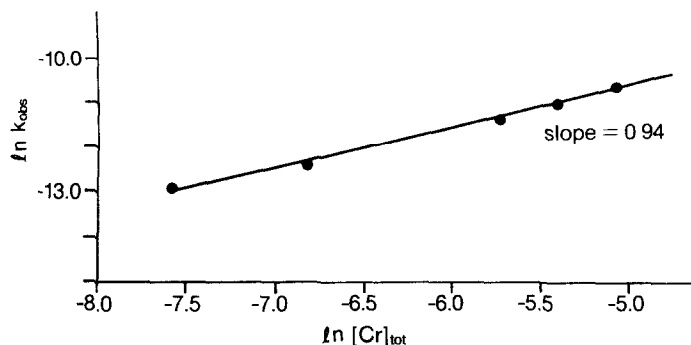
Fig. 4. Plot of the \ln k_{\text{obs}} versus \ln[\text{Cr}_{\text{tot}}] at 135°C under 100 p.s.i. \text{H}_2 pressure in hexane with [methyl linoleate] = 0.045 M.
