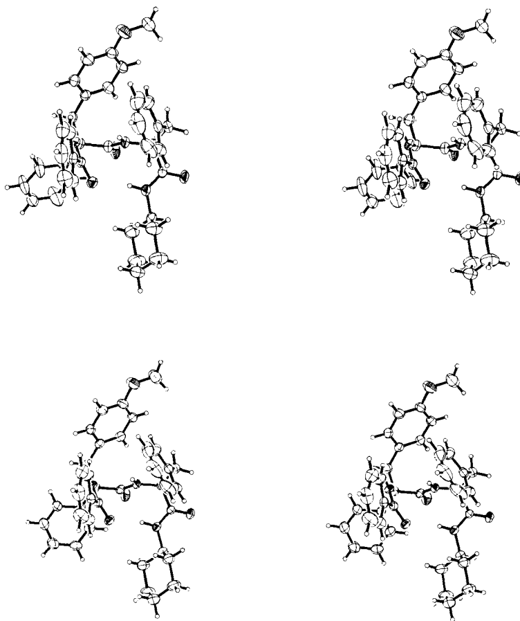
Fig. 3. Stereoplot (ORTEP) of 4c and 4c' (two independent molecules in the asymmetric unit)
